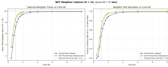
Figure 9. Mean filled neighbor slots and slot saturation versus cone \Delta R for K = 10 .
